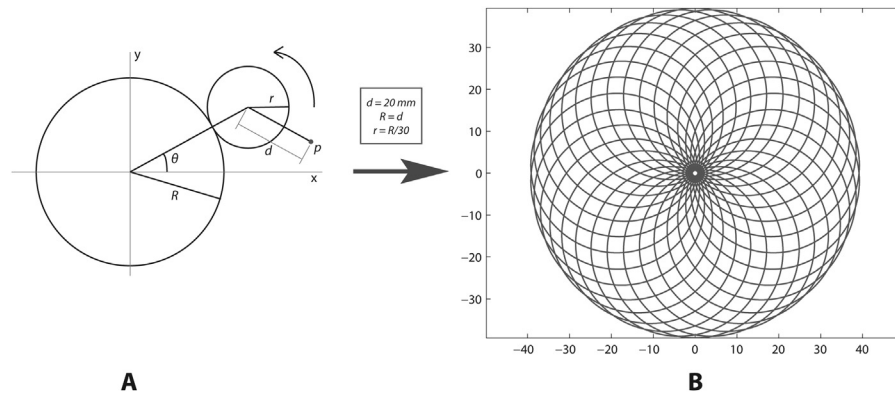
Supplemental Figure 1 Genesis of an epitrochoid curve. (A) Analytically, an epitrochoid is a curve traced by a point p attached to a circle of radius r rolling around the outside of a fixed circle of radius R , where the point p is a distance d from the center of the exterior circle. The parametric equation for an epitrochoid curve is \begin{pmatrix} x(\theta) = (R + r)\cos\theta - d\cos\left(\frac{R+r}{r}\theta\right) \\ y(\theta) = (R + r)\sin\theta - d\sin\left(\frac{R+r}{r}\theta\right) \end{pmatrix} , with parameter \theta ranging from 0 to 2\pi . For a disk occluder of radius S , the parameters in the equation can be approximated as follows: R = \frac{S}{2} ; d \cong R ; r \ll R . (B) N samples of the parameter \theta were generated and used for simulation and plotting of the epitrochoid curve in a custom-written MATLAB routine. This figure shows an example of the output when simulating an input radius S = 40 \text{ mm} , sample size n = 10,000 , and r = R/30 . The value of r determines the density of the curve, with higher mesh densities for a smaller radius r .
